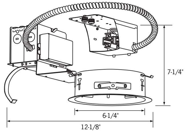
Ceiling Opening: 6-1/2"
