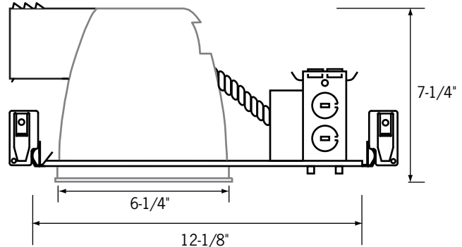
Shown with CST Series Reflector Ceiling Opening: 6-1/2" Plaster frame: 7-5/8" by 12-1/8" (less bar hangers)
