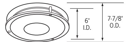
CTR6426H-P Floating Ring with White Reflector, 1-1/2" Drop, 3-1/2" Center Hole.
