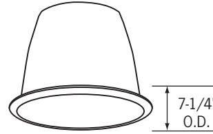
CST6422H-(CLR, PL) Reflector CST6423H-(CLR, PL) 90° Wall Wash Kicker Finishes: -CLR (Clear), -PL (Matte Platinum)
