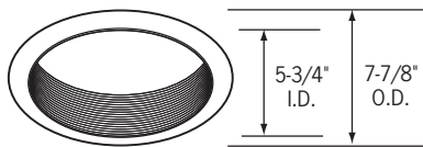
CTR6421H-B Black Baffle, Clear Reflector, Black Trim Ring
