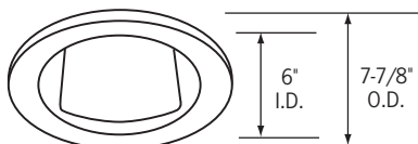
CTR6423H-CLR Wall Wash Kickplate, Clear Reflector, White Plastic Trim Ring
