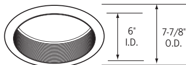
CTR6427H-P Black Baffle Trim
