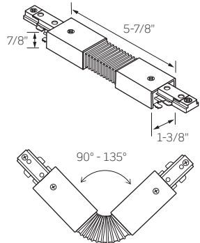
LA-203 Series Flexible Connector Allows wall to ceiling or pitched ceiling applications; ±90° max. horizontal range, ±135° max. vertical range
